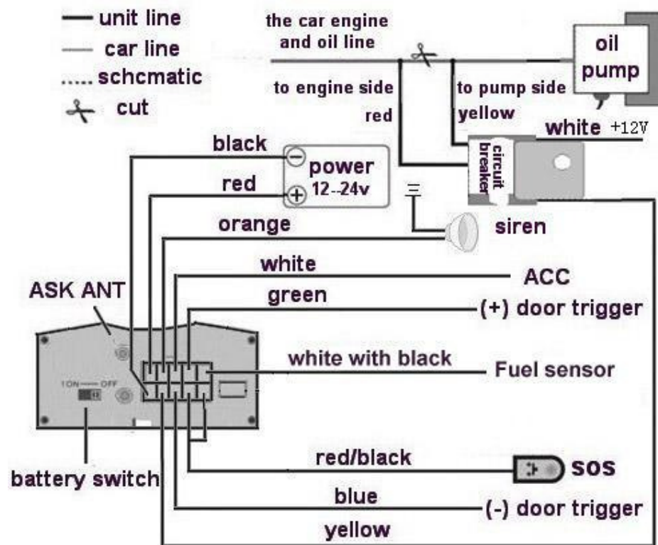
Wiring diagram
